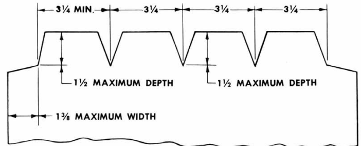
NOTCHING HEADS
